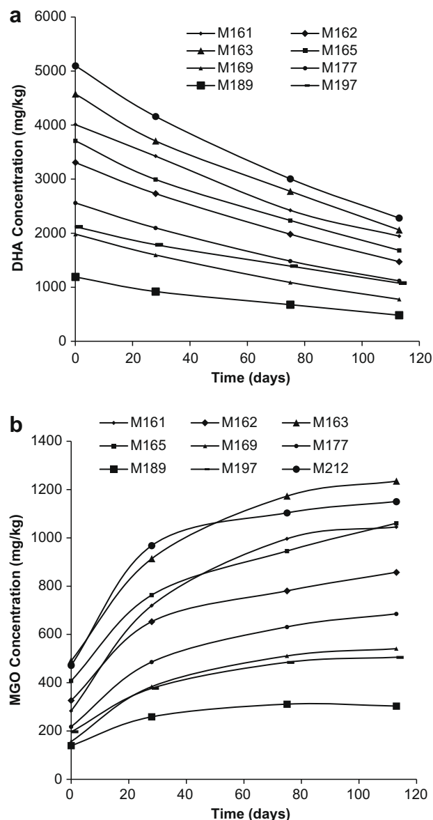
Figure 2. (a) Disappearance of dihydroxyacetone (DHA) in freshly produced honeys with time of storage at 37 °C. (b) Appearance of methylglyoxal (MGO) in freshly produced honeys with time of storage at 37 °C.
