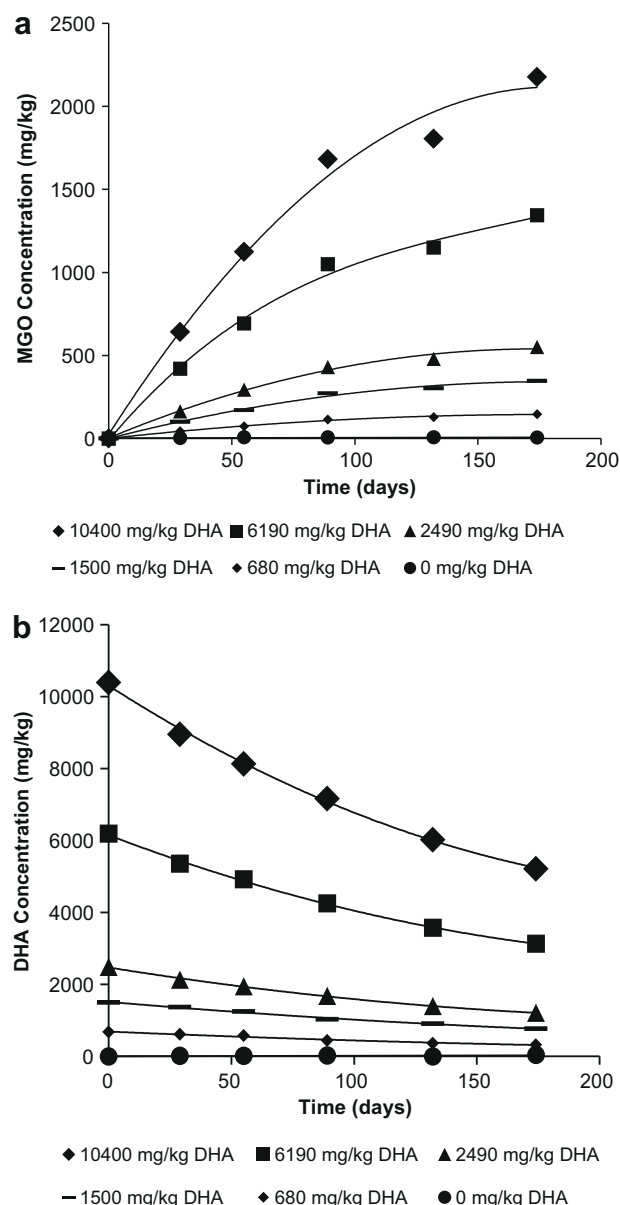
Figure 3. (a) Methylglyoxal concentrations (mg/kg) over time for a series of clover honey samples incubated at 37 °C in the presence of various initial concentrations of dihydroxyacetone (DHA). (b) Dihydroxyacetone concentrations (mg/kg) over time for a series of clover honey samples incubated at 37 °C in the presence of various initial concentrations of dihydroxyacetone.
