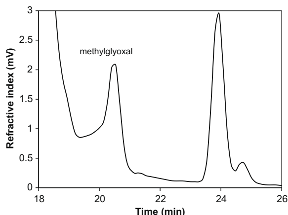
Figure 1. HPLC chromatogram of a UMF 30 + manuka honey: expanded view to show methylglyoxal and the peak at ~24 min, which was isolated.
